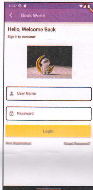
Fig 1: Login Screen
